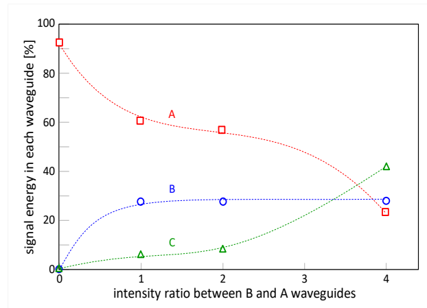
Figure 15. Energy stored inside each channel for an increasing power of channel B. In this case channel A and channel C are written with the same power.
