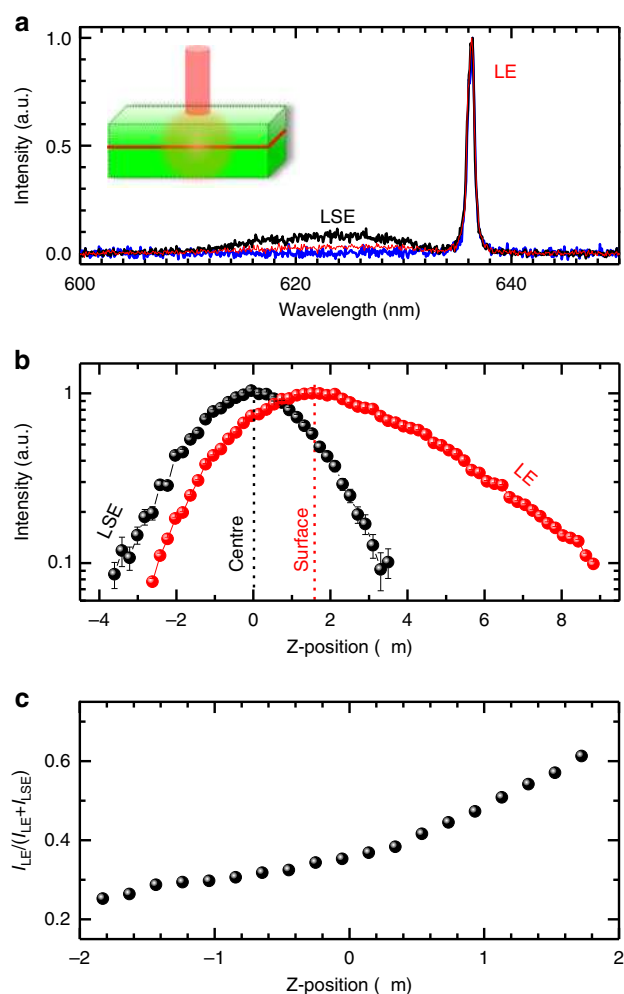
Fig. 3 Confocal photoluminescence scanning along Z-direction. a Normalised photoluminescence spectra collected at the cavity centre (black), surface (red) and 5.1 \mu\text{m} (i.e., the distance above the cavity centre, blue), respectively. The used excitation power is 100 nW. The inset shows the emission schematic. b Comparison of normalised integrated intensities of the lasing emission (LE) and the leaked spontaneous emission band (LSE) at various Z-positions. Error bars are extracted from single and double Lorentzian fits to the confocal spectra. c The lasing intensity ratio to the detected total light output as a function of Z-position. The defined Z-direction is perpendicular to the sample surface. I_{\text{LE}} and I_{\text{LSE}} represent the integrated intensities of LE and LSE, respectively
