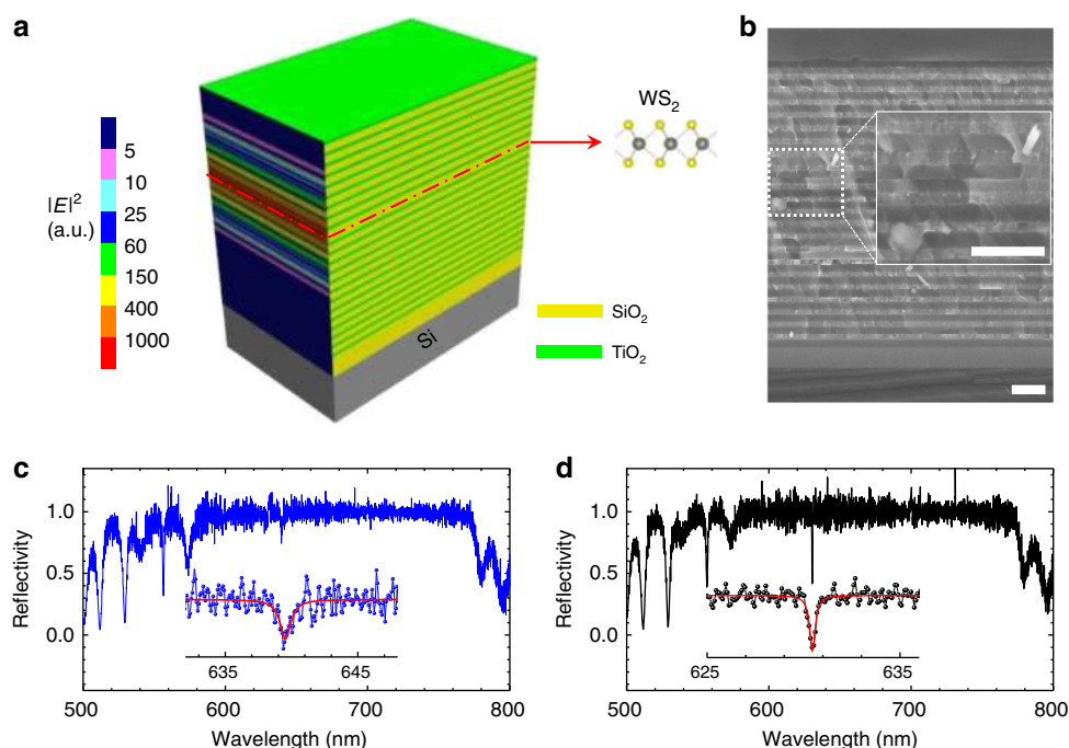
Fig. 1 Structure of a 2D semiconductor embedded microcavity and its reflection. a Schematic of a 2D semiconductor embedded microcavity on the \text{SiO}_2/\text{Si} substrate consisting of 12.5 pairs of bottom \text{TiO}_2/\text{SiO}_2 distributed Bragg reflectors (DBRs), half-wavelength-thick \text{SiO}_2 cavity with embedded monolayer \text{WS}_2 and 8.5 pairs of top DBRs. b Representative scanning electron microscope image of the cross-section. The inset shows the zoom-in image. Scale bars in b and its inset represent 500 nm. c, d Reflection spectra of monolayer \text{WS}_2 embedded microcavity (in blue) and the blank microcavity region (in black) in the spectral range from 500 to 800 nm, respectively; The insets show the enlarged spectra together with the Lorentzian fits (in red) in the cavity-mode regions, respectively
