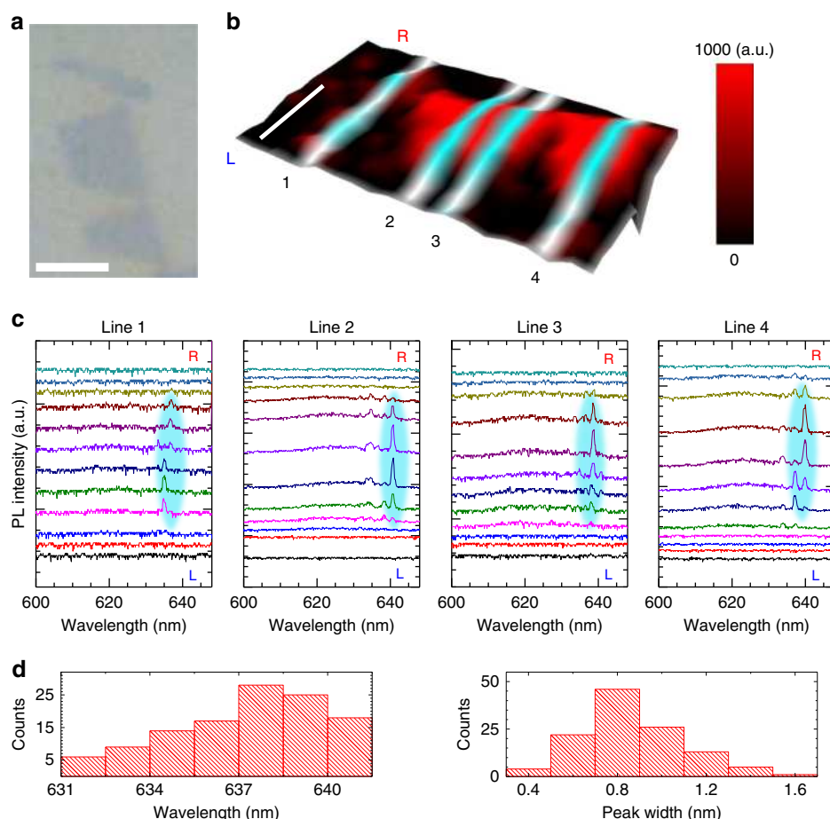
Fig. 4 2D lasing from monolayer \text{WS}_2 flakes. a Optical image of three 1L- \text{WS}_2 flakes on the half cavity and b spatially resolved PL intensity image of the complete microcavity samples. The PL intensity is integrated from 600 to 645 nm. Line profile analysis was carried out along the marked lines. L and R indicate left and right sides, respectively. The scale bars represent 3 \mu\text{m} . c The series of PL spectra taken along four marked lines with a step size of 500 nm. The colour traces from bottom to top correspond to the spectra taken from left to right of each scanning line in b . The dominant lasing modes are highlighted in cyan. d Statistics of positions and widths of narrow emission bands in 67 spectra sampling from three flakes
