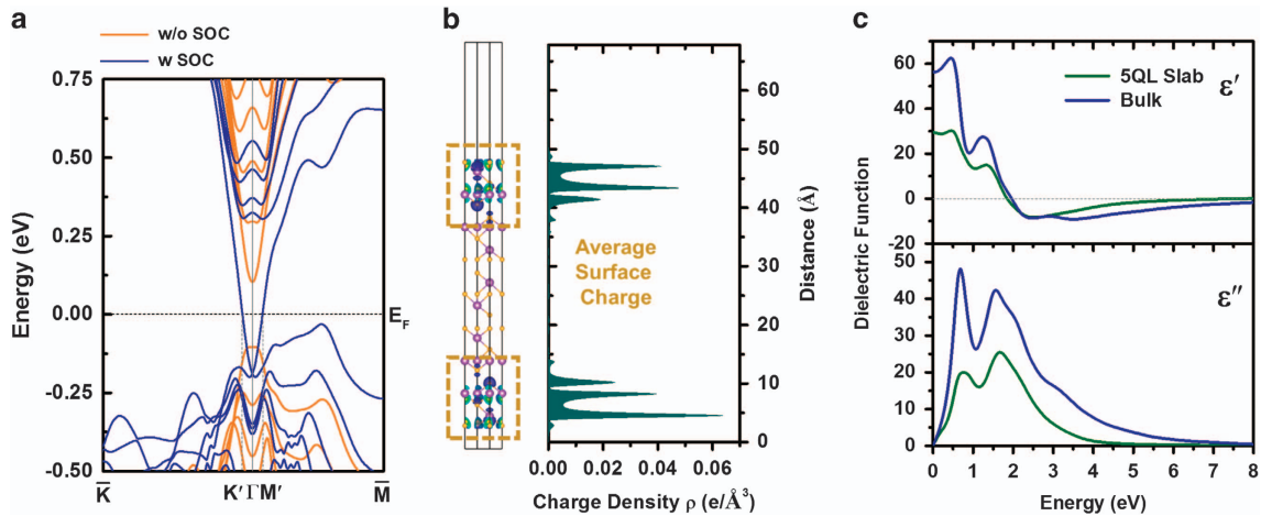
Figure 4 (a) Band structure of 5QL Bi 2 Se 3 slab without and with inclusion of spin-orbit coupling effects (the horizontal dashed line indicates the Fermi energy level and K'-M' the region of occupied surface states). (b) Three- and one-dimensional charge density distribution of conducting surface states; all occupied orbitals below the Fermi level and their degeneracy (Supplementary Figure 7) were considered to calculate the average charge density. (c) Comparison between real and imaginary parts of the dielectric functions of bulk and 5QL Bi 2 Se 3 slab with spin-orbital coupling (SOC).
