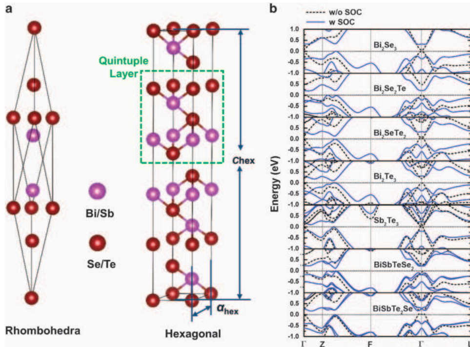
Figure 1 (a) Crystal structure of BiSb 1-x Te y Se 1-y (BSTS) compounds exhibiting topological insulator (TI) behavior (rhombohedral and equivalent hexagonal lattice cell, with a quintuple layer (QL) shown by the green rectangle); (b) band structures of bulk BSTS compounds calculated with and without account of spin-orbit coupling.
