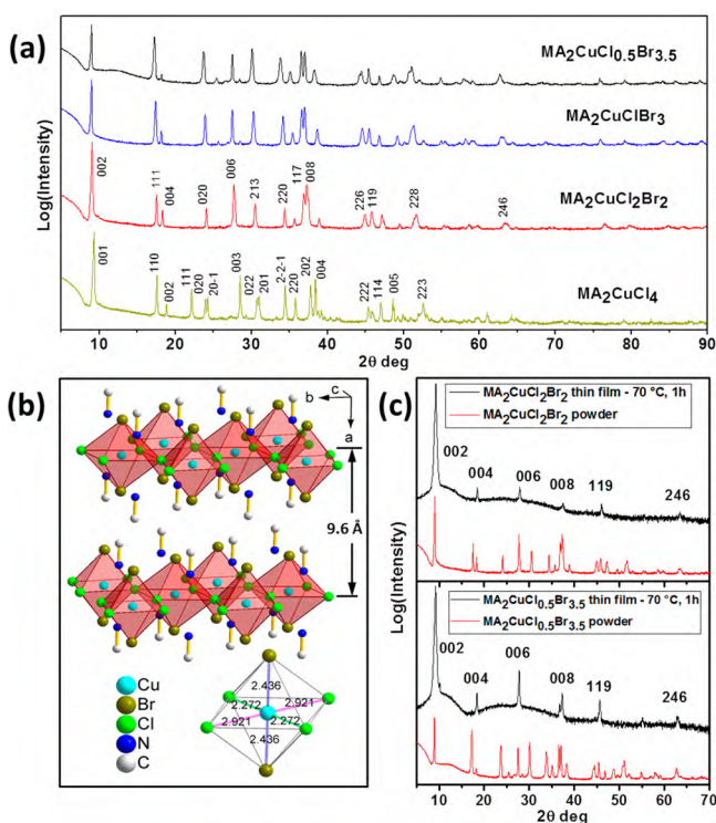
Figure 1. XRD characterization of 2D copper-based perovskites: (a) powder XRD of MA 2 CuCl 4 (yellow), MA 2 CuCl 2 Br 2 (red), MA 2 CuClBr 3 (blue), and MA 2 CuCl 0.5 Br 3.5 (black); (b) crystal structure of MA 2 CuCl 2 Br 2 , showing the alternation of organic and inorganic layers and the Cu–X bond lengths in the inorganic framework (structural data taken from ICSD No. 110677); 48 (c) thin film XRD of MA 2 CuCl 2 Br 2 (upper) and MA 2 CuCl 0.5 Br 3.5 (lower) compared to their respective powders, showing strong preferential orientation toward the 00l direction.
