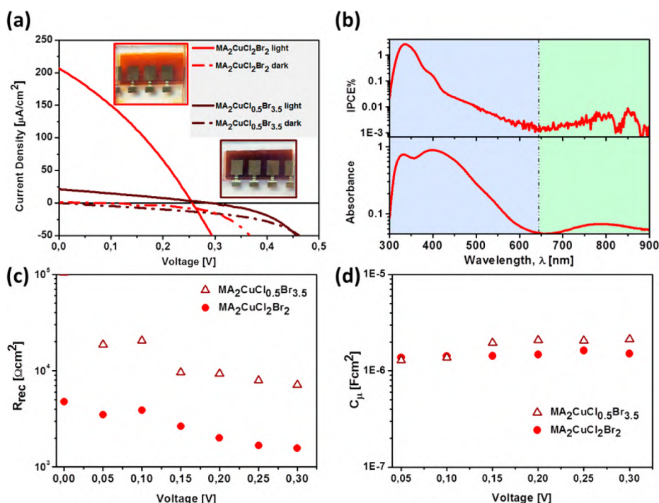
Figure 5. (a) I – V curve of solar cells sensitized with \text{MA}_2\text{CuCl}_2\text{Br}_2 (red) and \text{MA}_2\text{CuCl}_{0.5}\text{Br}_{3.5} (brown) under 1 sun of light illumination. The dashed red and brown lines represent the dark current; (b) photocurrent measurement performed on a device sensitized with \text{MA}_2\text{CuCl}_2\text{Br}_2 (upper) compared to the perovskite absorption spectrum. (c) Recombination resistance and (d) chemical capacitance extracted from the fitting of the IS spectra measured under 1 sun of illumination.
