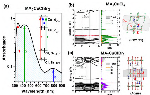
Figure 3. (a) Representation of the electronic transitions for \text{MA}_2\text{CuClBr}_3 : charge-transfer transitions 1 and 2 ( \text{Cl, Br } p\sigma \rightarrow \text{Cu } d_{x^2-y^2} and \text{Cl, Br } p\pi \rightarrow \text{Cu } d_{x^2-y^2} ) and d–d transition 3 ( \text{Cu } d_{xy} \rightarrow \text{Cu } d_{x^2-y^2} ; see Figure S11, Supporting Information for more details); electronic band structure, density of states, and unit cell structure of the perovskite compounds (b) \text{MA}_2\text{CuCl}_4 and (c) \text{MA}_2\text{CuClBr}_3 investigated by DFT simulation.
