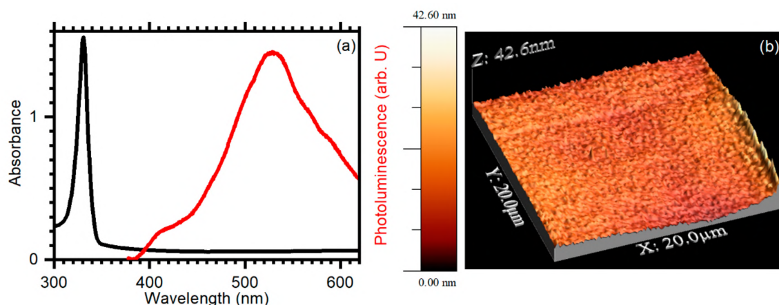
Figure 1. (a) (EDBE)PbCl 4 absorbance (black line) and photoluminescence (red line) spectra. (b) atomic force microscopy (AFM) micrograph of an (EDBE)PbCl 4 thin film with thickness of 40 nm deposited on fused silica substrate.
