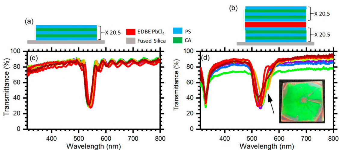
Figure 2. Schematic (a,b) and transmittance spectra (c,d) of a polymer half microcavity (a,c) and of a microcavity where the defect layer consist in an (EDBE)PbCl 4 thin film (b,d). The inset of panel (d) is a digital photograph of the microcavity.
