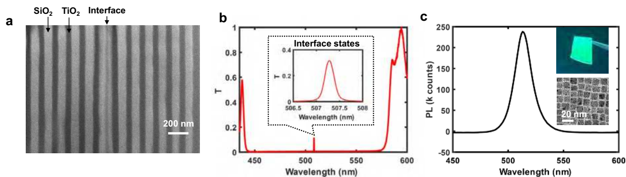
Fig. 3 | Topological microcavity and gain medium. a Cross-sectional scanning electron microscope (SEM) image of the 1D microcavity consisting of 20 alternating layers of \text{TiO}_2 and \text{SiO}_2 and on each side of the interface. b Measured transmission spectrum of the 1D topological cavity. The high-Q transmission peak (Q=2000) at 507.3 nm, arising from the interface state, is magnified in the inset. c Room
