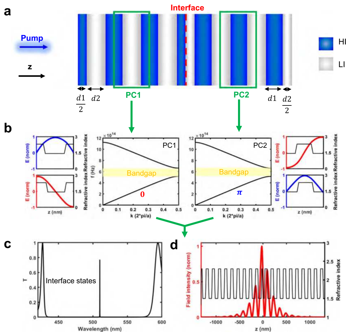
Fig. 1 | Design principles of a 1D topological microcavity. a Schematic of a one-dimensional (1D) topological microcavity formed by interfacing two photonic crystals (PC1 and PC2) composed of alternative high index (HI) and low index (LI) layers. The inversion center of PC1 is chosen to be within the LI layer, while the inversion center of PC2 is within the HI layer, as highlighted by the green boxes. b The calculated optical band structures of PC1 and PC2 are identical but have
