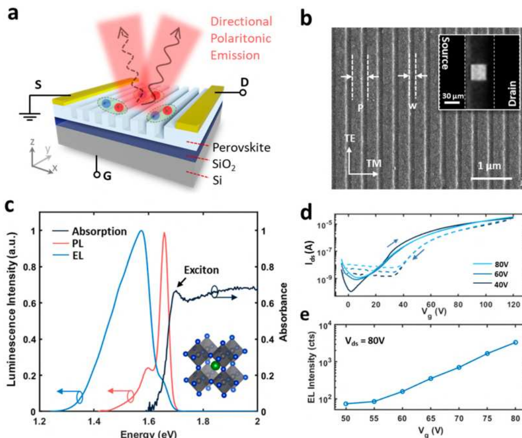
Figure 1. Electrically driven polaritonic perovskite metasurface. (a) Schematic of the electrically driven perovskite metasurface with tunable polaritonic emission. A resonant dielectric metasurface is monolithically fabricated within the active region of the transistor between the source (S) and drain (D) electrodes, leading to strong coupling of photonic modes and electrically injected excitons. The resulting polaritonic EL intensity and directionality can be controlled by the gate (G) and source-drain biases, respectively. (b) SEM image of the perovskite nanobeam array fabricated by FIB lithography within the active region between the top S-D electrodes. The perovskite nanobeams had a period (P) ranging from 380 and 400 nm, a height of 125 nm, and a spacing (w) of 100 nm. The optical microscope image of the device operating at V_g = \pm 80 V and V_{ds} = 80 V in the inset shows the region of enhanced EL corresponding to the nanopatterned region of the square metasurface. (c) PL and absorption spectra of the MAPbI 3 perovskite compared to the EL spectrum of the unpatterned LET at 78 K. The crystal structure of the MAPbI 3 perovskite is shown in the inset, where green, black, and blue spheres represent MA + , Pb 2+ , and I − ions, respectively. (d) Transfer characteristics of the MAPbI 3 LET obtained in the forward and backward sweeping direction of gate bias with V_{ds} = 40, 60, and 80 V. (e) Peak EL intensity dependence on AC gate bias with V_{ds} = 80 V.
