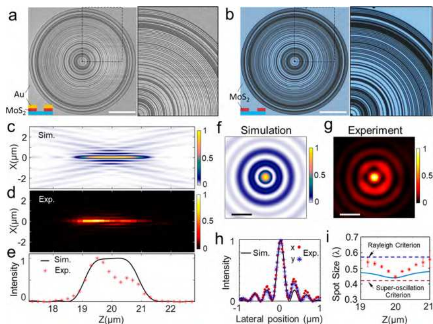
Figure 4. MoS 2 -based supercritical lens. (a) SEM and (b) microscopic images of fabricated lens before and after removing the top gold layer. Scale bars: 20 \mu\text{m} . (c) Simulated and (d) experimental intensity profiles at the x - z plane. In d, the measured needle is not well-mapped because of the slight deviation of optical axis during the z -direction scanning. So, we provide the x - z intensity profiles around the focal plane, which is extracted from the x - y intensity profiles at different z -cut planes from z = 19 \mu\text{m} to z = 21 \mu\text{m} . (e) Comparison of on-axis intensity between simulation and experiment. (f) Simulated and (g) measured spot at the focal plane. Scale bars: 500 nm. (h) Simulated and experimental line-scanning intensity profiles. The x - and y -scanning profiles in measured spot are shown by red dots and blue stars, respectively. (i) Spot size of optical needle from z = 19 \mu\text{m} to z = 21 \mu\text{m} . The Rayleigh and superoscillation criteria are given, respectively, by 0.515\lambda/\text{NA} (FWHM) and 0.38\lambda/\text{NA} . The experimental results (labeled by red stars) showed subdiffraction focusing below Rayleigh criterion. The blue curve is simulated focusing spot size.
