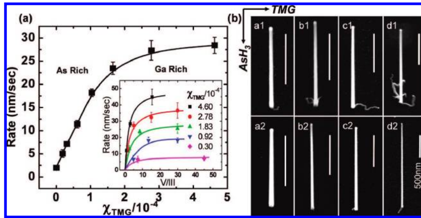
Figure 4. Dependence of NW growth rate and morphology on TMG and AsH_3 molar fractions. (a) NW growth rate as a function of TMG molar fraction with fixed \chi_{AsH_3} = 1.38 \times 10^{-3} ; the inset shows the growth rate as a function of V/III ratio for different TMG molar fractions. The continuous lines are a guide to the eye. (b) Morphology of GaAs NWs grown at 417 °C with different TMG and AsH_3 molar fractions. NWs in the first row were grown at low AsH_3 molar fraction of 1.38 \times 10^{-3} and TMG molar fractions of (a1) 0.92 \times 10^{-4} , (b1) 1.83 \times 10^{-4} , (c1) 2.78 \times 10^{-4} , and (d1) 4.60 \times 10^{-4} ; keeping the same TMG setting as used in the first row, NWs in the second row were grown with AsH_3 molar fractions of (a2) 2.80 \times 10^{-3} , (b2) 5.60 \times 10^{-3} , (c2) 4.20 \times 10^{-3} , and (d2) 7.22 \times 10^{-3} .
