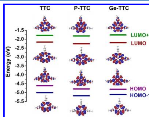
Figure 3. Frontier molecular orbital energies and electronic density distribution of molecules TTC, P-TTC, and Ge-TTC.
