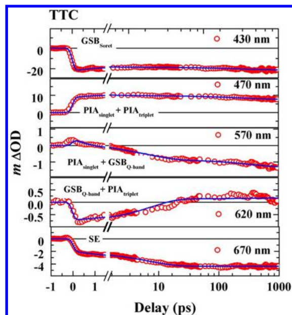
Figure 6. TA kinetics of TTC at selected probe wavelengths. (red \circ ) Experimental data. (blue) Theoretical fits after global analysis.
