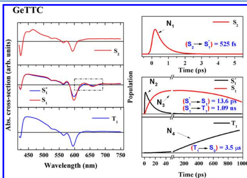
Figure 12. (left) Basis spectra for Ge-TTC obtained from the global fitting procedure. The dotted rectangle represents the spectral region where S_1^* differs from S_1 ; (right) the decay dynamics of different species with rate constants.
