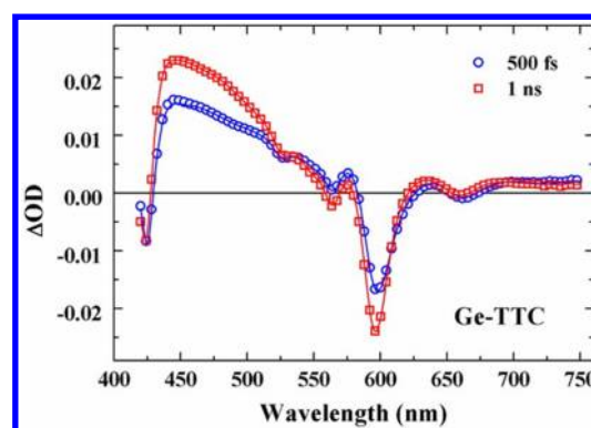
Figure 13. fs-TA spectra of Ge-TTC at a pump–probe delay of 500 fs and 1 ns demonstrating an excellent agreement of the global analysis fit (solid curve) with the experimental data (O,□).
