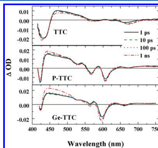
Figure 4. fs-TA spectra of TTC, P-TTC, and Ge-TTC recorded at 1 ps, 10 ps, 100 ps, and 1 ns.
