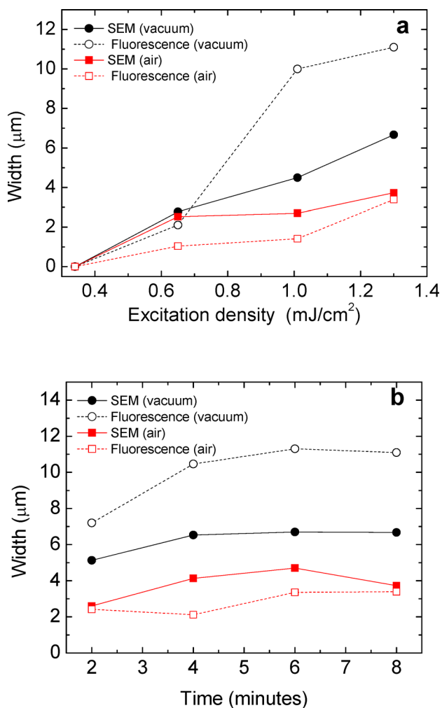
Figure 4. Footprint width in a vacuum and in air as detected from SEM images and fluorescence maps as a function (a) of the excitation density under continuous laser pumping and (b) the time at 1.30 \text{ mJ cm}^{-2} .
