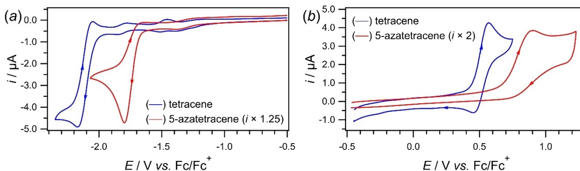
Figure 8. Comparison of (a) first reduction and (b) first oxidation process of 1 \text{ mM} 5-azatetracene and tetracene. Cyclic voltammograms were recorded in DCM containing 0.1 \text{ M } n\text{Bu}_4\text{NPF}_6 at a scan rate of 0.1 \text{ V s}^{-1} and using a 1 \text{ mm} diameter GC working electrode at 298 \pm 2 \text{ K} in a Faraday cage.
