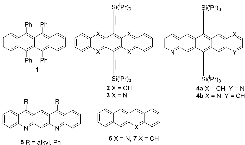
Figure 1. Chemical structures of acenes and heteroacenes.
