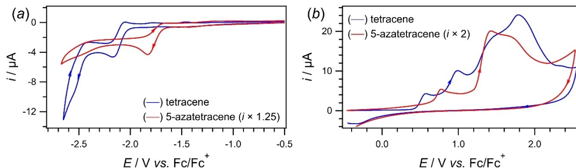
Figure 7. Cyclic voltammograms obtained in DCM containing 0.1 \text{ M } n\text{Bu}_4\text{NPF}_6 at a scan rate of 0.1 \text{ V s}^{-1} and using a 1 \text{ mm} diameter GC working electrode at 298 \pm 2 \text{ K} in a Faraday cage. (a) Reduction processes of 1 \text{ mM} 5-azatetracene and tetracene. (b) Oxidation processes of 1 \text{ mM} 5-azatetracene and tetracene.
