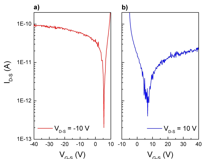
Figure 9. Representative p-type (a) and n-type (b) transfer characteristics measured at drain-source bias voltage of V_{D-S} = \pm 10 V. V_{G-S} is the applied gate-source voltage and I_{D-S} is the measured drain-source current.
