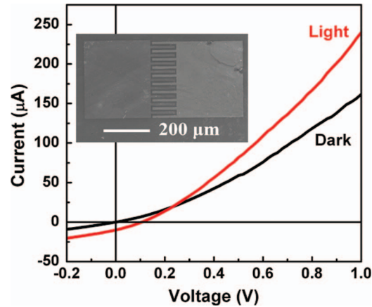
FIG. 5. Current-voltage curves of the Pt/STO/Al Schottky junction made of the S75 sample measured either in dark and under the illumination of a simulated solar light AM 1.5 ( 100 \text{ mW/cm}^2 ). The inset shows a scanning electron microscopy image of the device with interdigitated semitransparent Pt (left) and Al (right) electrodes.
